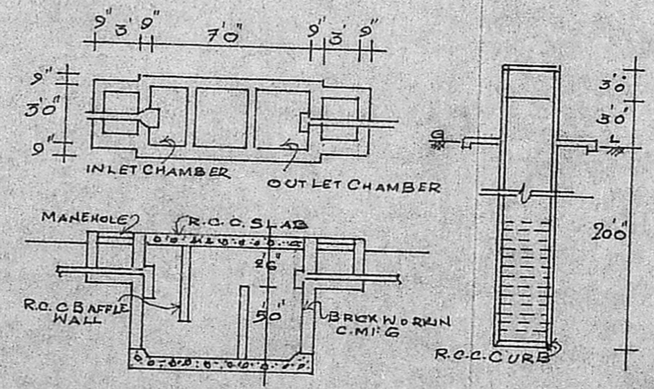
DETAILS OF SEPTICTANK & 4 DIA WELL
